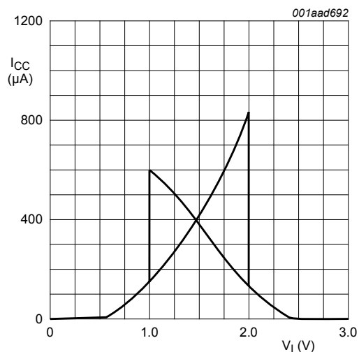
Fig. 8. Typical transfer characteristics; V_{CC} = 3.0 \text{ V}
